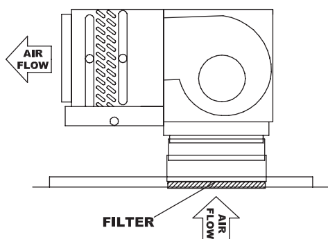
HPP BOTTOM RETURN WITH TELESOPING BOTTOM PANEL
