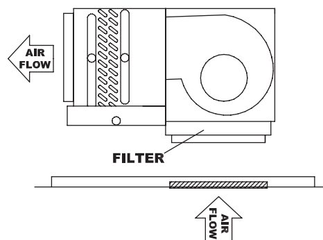
HPP BOTTOM RETURN W/BOTTOM CEILING PANEL
