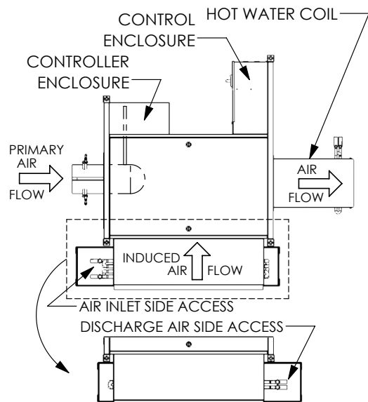
CRC ARRANGEMENT 1 LEFT HAND CONTROL UNIT LEFT HAND HW COIL
