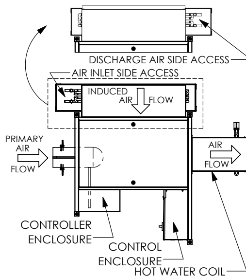
CRC ARRANGEMENT 4 RIGHT HAND CONTROL UNIT LEFT HAND HW COIL
