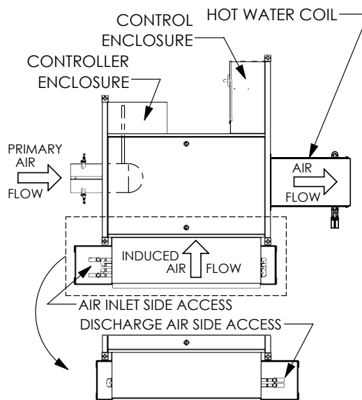
CRC ARRANGEMENT 2 LEFT HAND CONTROL UNIT RIGHT HAND HW COIL
