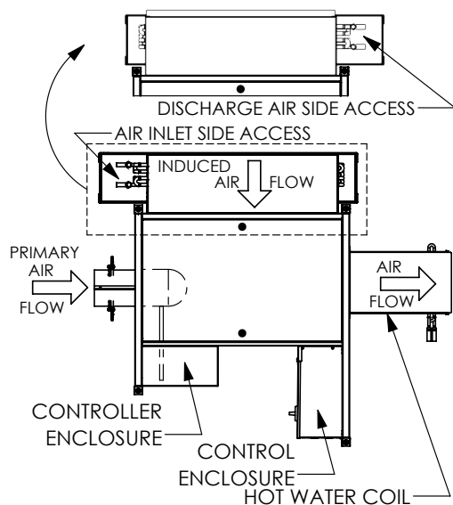
CRC ARRANGEMENT 3 RIGHT HAND CONTROL UNIT RIGHT HAND HW COIL
