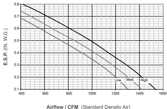
UNIT SIZE 1018, 1218, 1418
