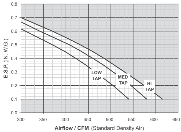
UNIT SIZE 1006
