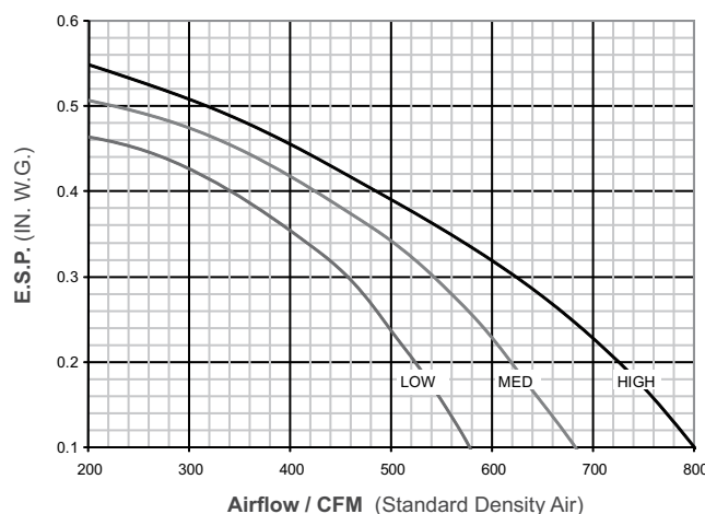
UNIT SIZE 0811, 1011, 1211
