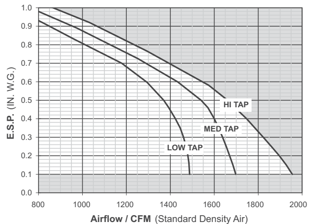
UNIT SIZE 1218
