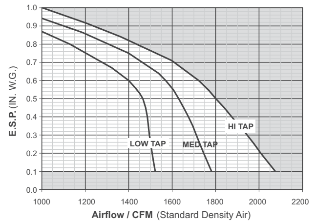
UNIT SIZE 1221
