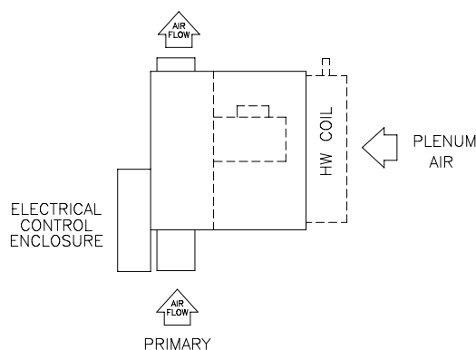
ARRANGEMENT 2 Left Hand Control Unit With Right Hand Hot Water Coil
