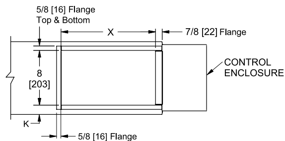
Discharge Air Opening Detail
